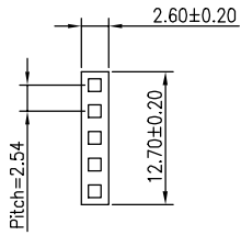
HOUSING
