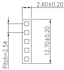
HOUSING
