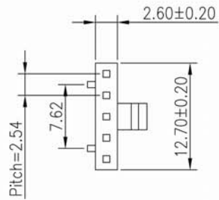
HOUSING (LOCKING)
