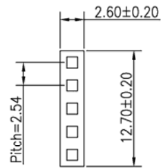
HOUSING
